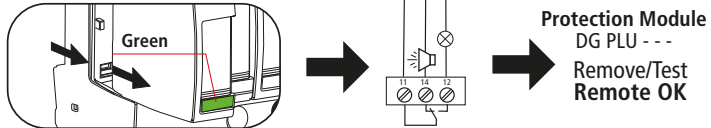
Fault Indication
