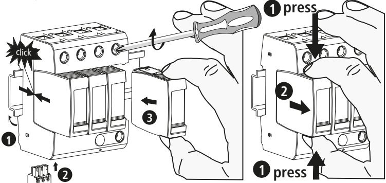
Mounting
